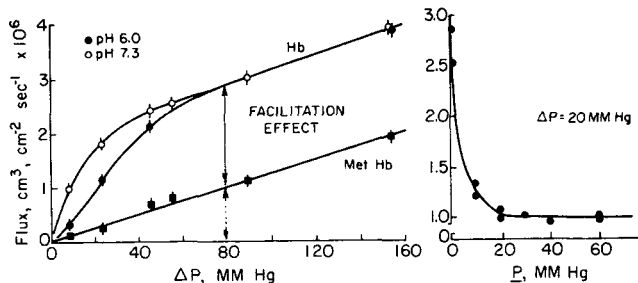
Fig. 2. Typical nonlinear flux patterns for carrier-mediated facilitated diffusion: a. Oxygen diffusion through hemoglobin solution, measured by O_2^{18} (Hemmingsen, 1962); b. Effect of back pressure on facilitated flux through hemoglobin solutions (Hemmingsen and Scholander, 1960).
