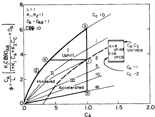
Fig. 11. Competitive carrier-mediated transport, two permeants competing for a single carrier. Regions showing uphill, hindered, and accelerated diffusion.
